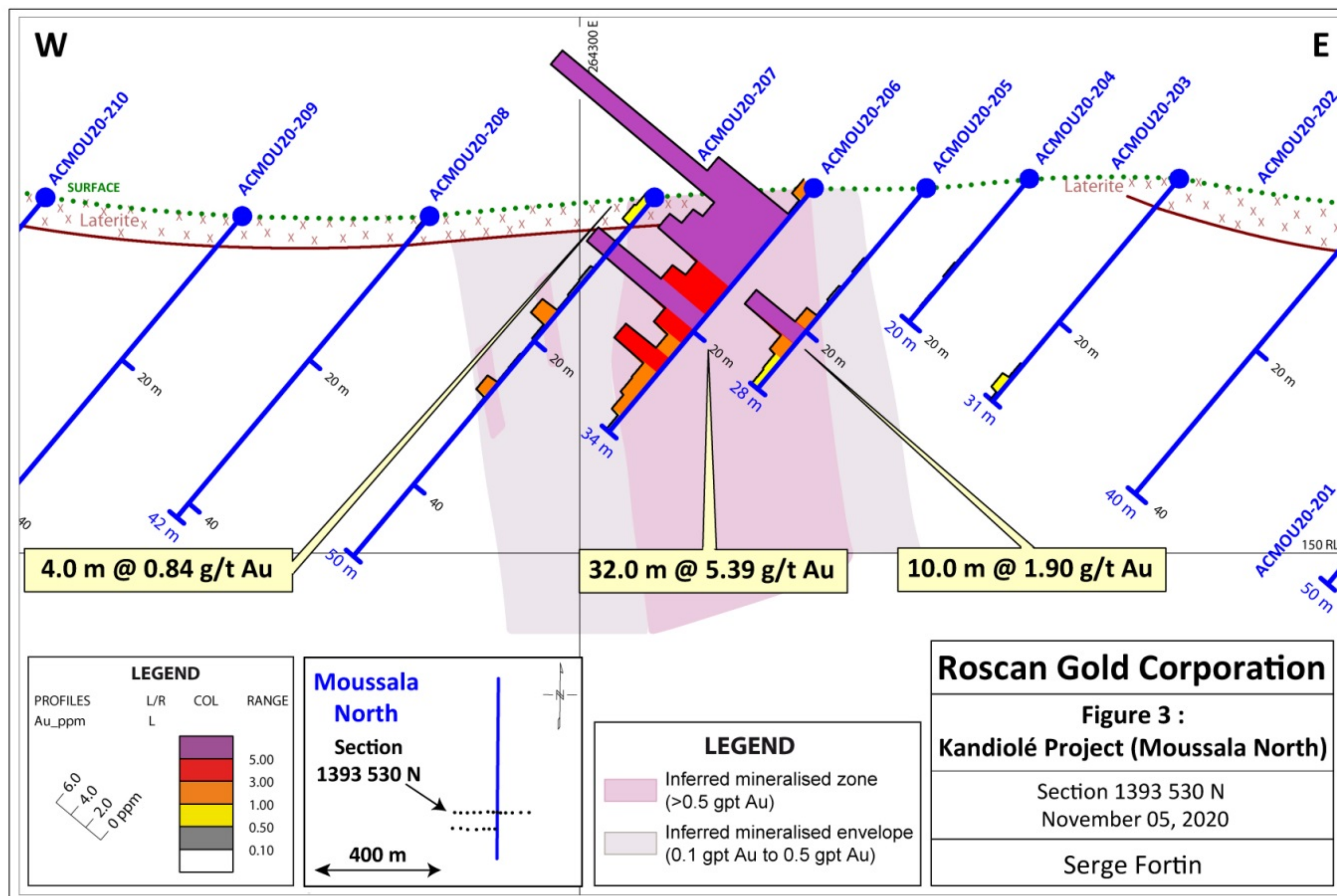
Cross Section at Moussala North
